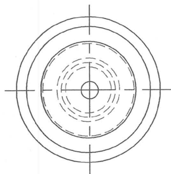
3/4" 或 1.5" Tri-Clamp 夾盤 3/4" or 1.5" Tri-Clamp Ferrule Connection
